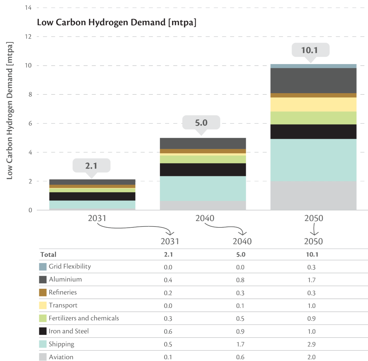
Figure 4 UAE Low Carbon Hydrogen Sectoral Demand from 2031 to 2050 in mtpa. Source: Fraunhofer CINES.
