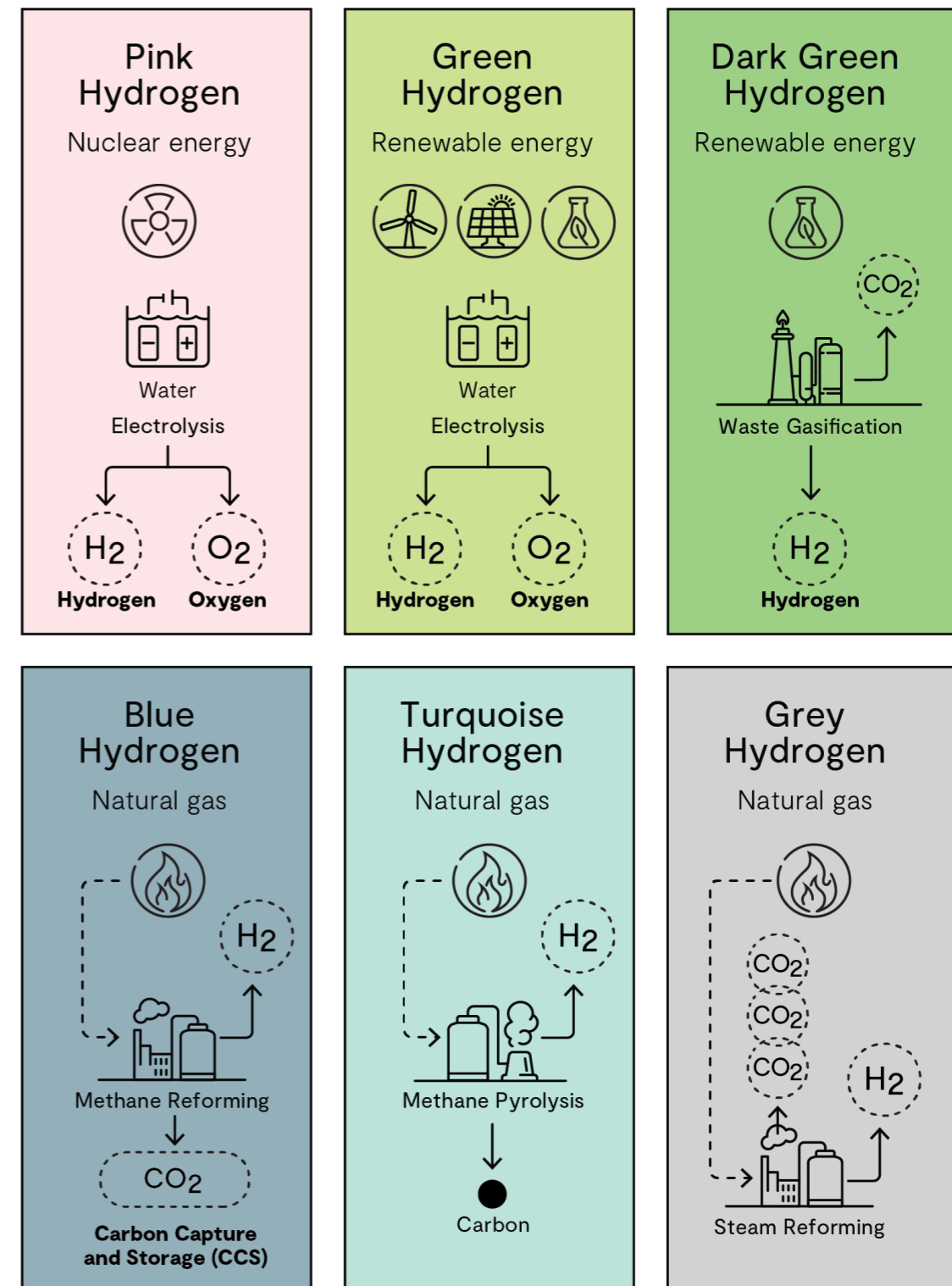
The different colours of hydrogen relevant to the UAE and how they are produced
