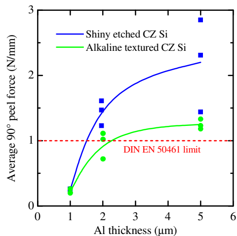
Fig. 4: Average values of the measured interconnect ribbons' 90 ^\circ peel forces of as a function of PVD Al thickness on shiny etched and alkaline textured silicon, respectively. The Al was electroless plated with about 1 \mu\text{m} Me. Lines are guides to the eye.
