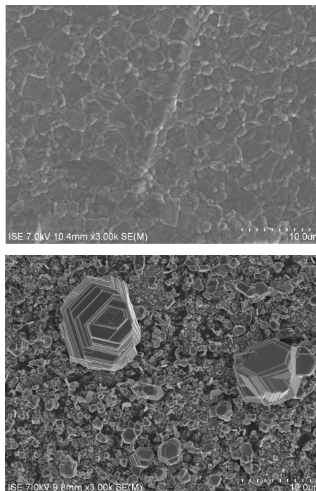
Fig. 1: Plan view SEM picture taken from 3 \mu\text{m} Al thermally evaporated on shiny etched Si before (top) and after (bottom) electroless metal deposition.
